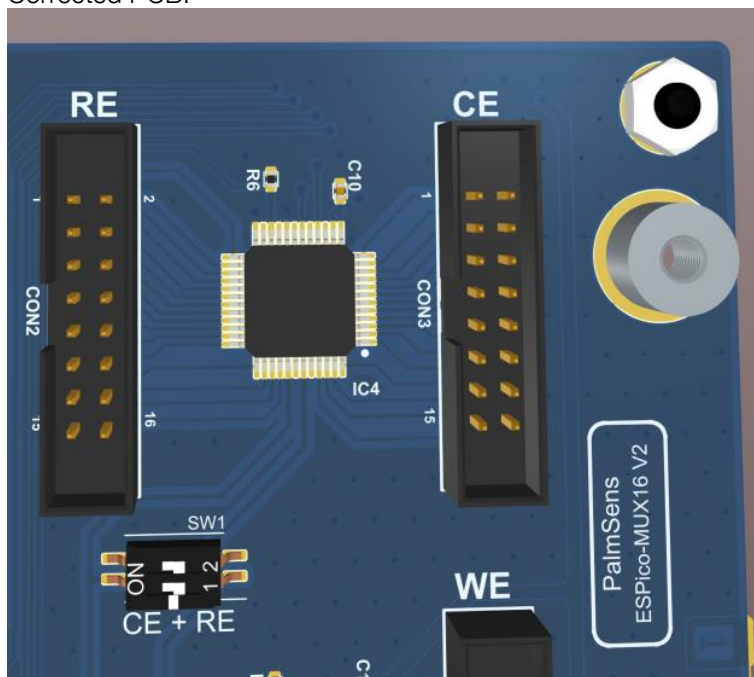
Corrected PCB:
